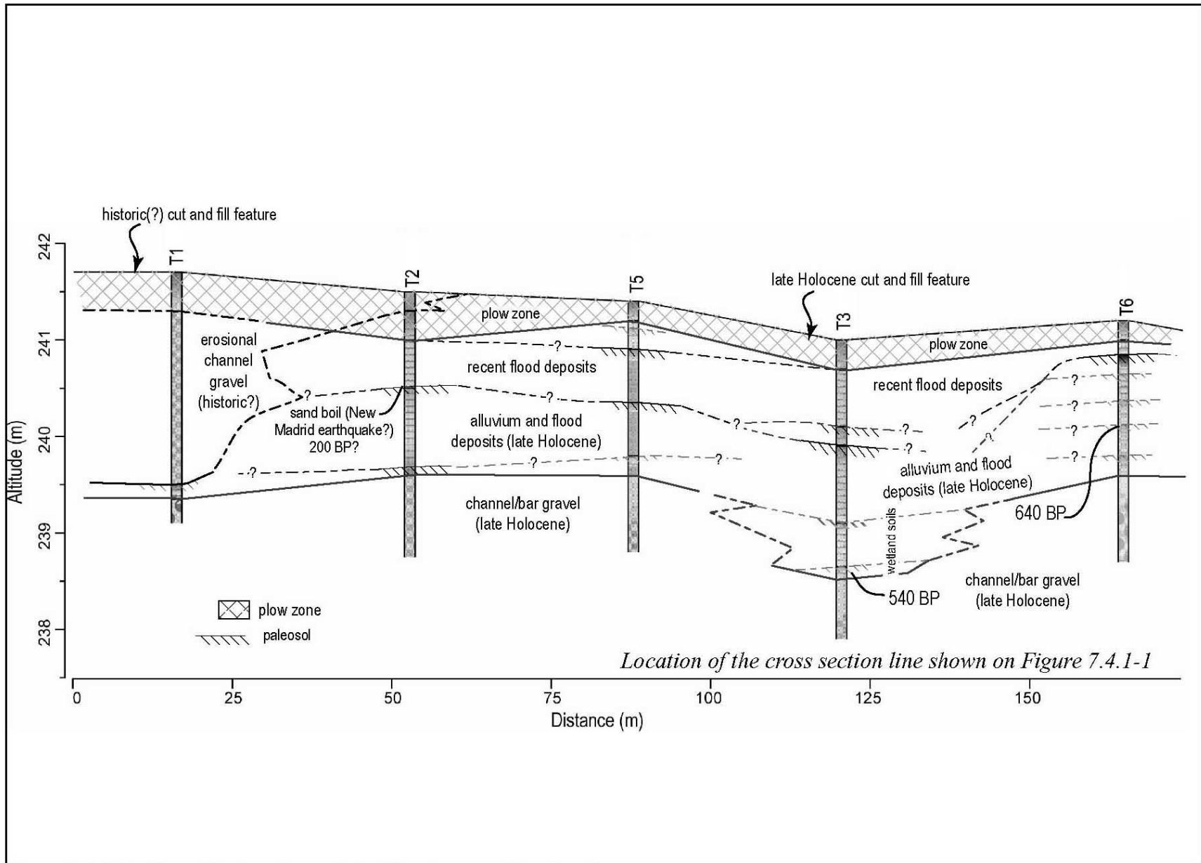
Figure 7.4.1-2. Cross Section through the City Property Test Locale
