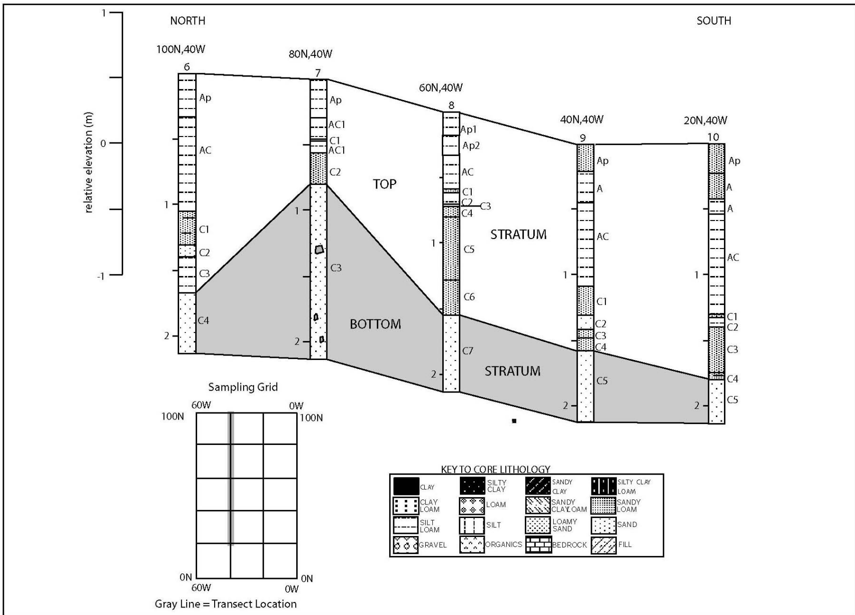
Figure 7.3.1-1. North-South Stratigraphic Cross-Section, City Property Test Locale
