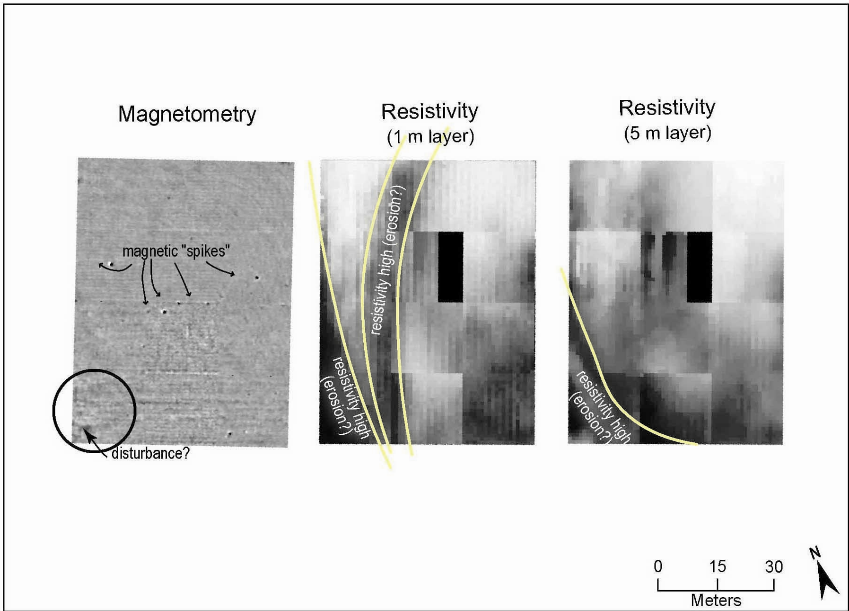
Figure 7.2.1-1. Magnetometry and Resistivity Data Plots, City Property Test Locale
